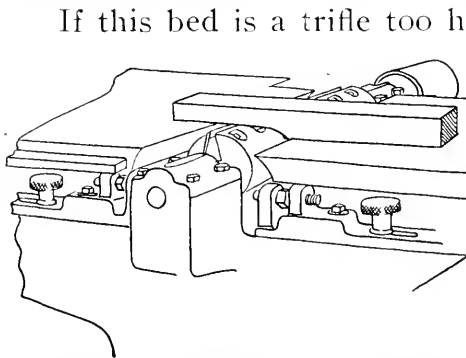
FIG. 136. SHOWING REAR TABLE SETTING OF JOINTER.
